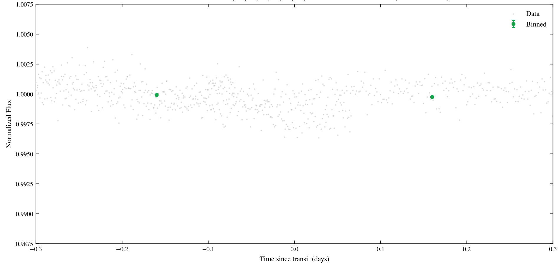
TIC 287196418 | Sectors: 53, 54, 55, 56, 57, 58, 59, 60 | Phase-Folded Transit (P = 63.92298 d)
