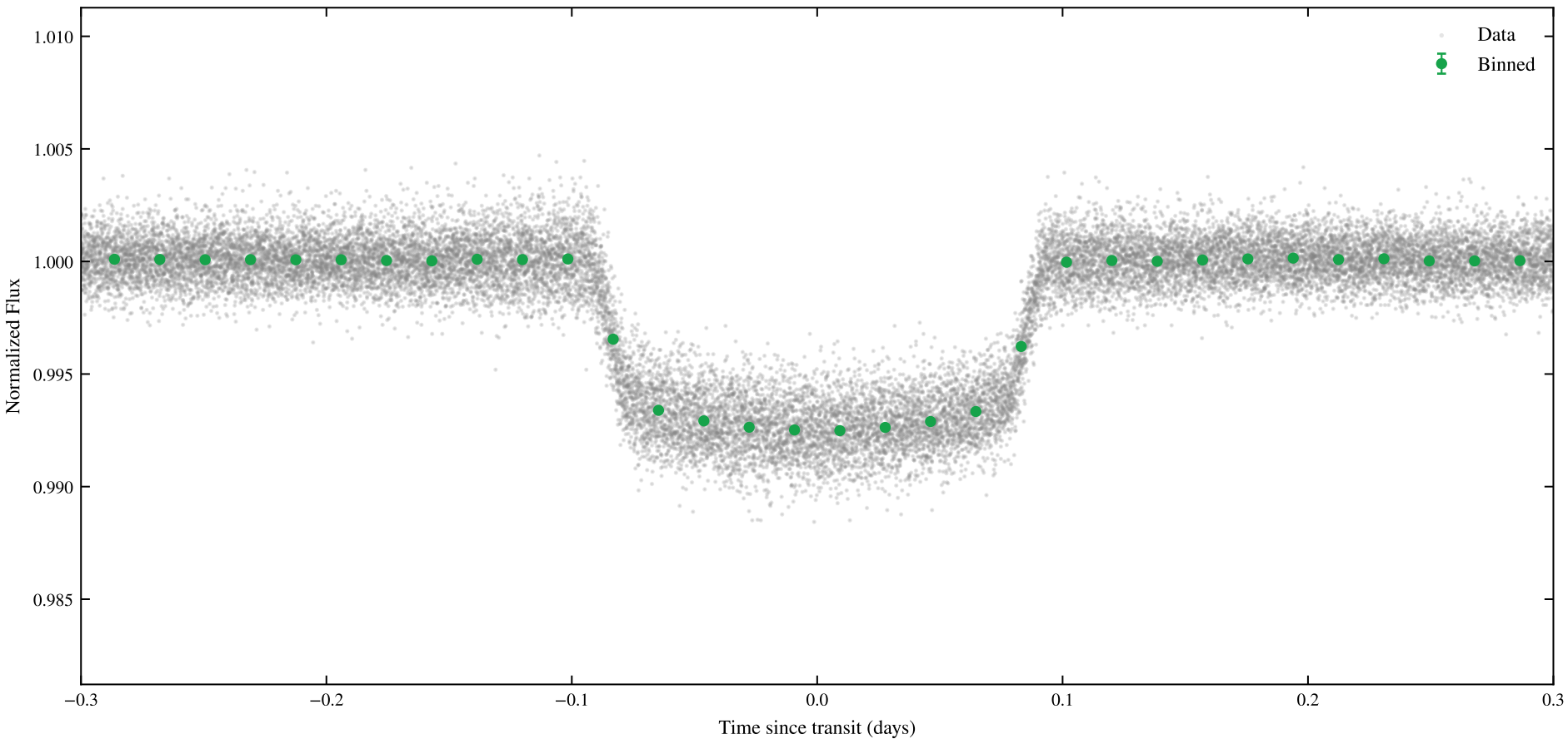
TIC 287196418 | Sectors: 53, 54, 55, 56, 57, 58, 59, 60 | Phase-Folded Transit (P = 3.69500 d)
