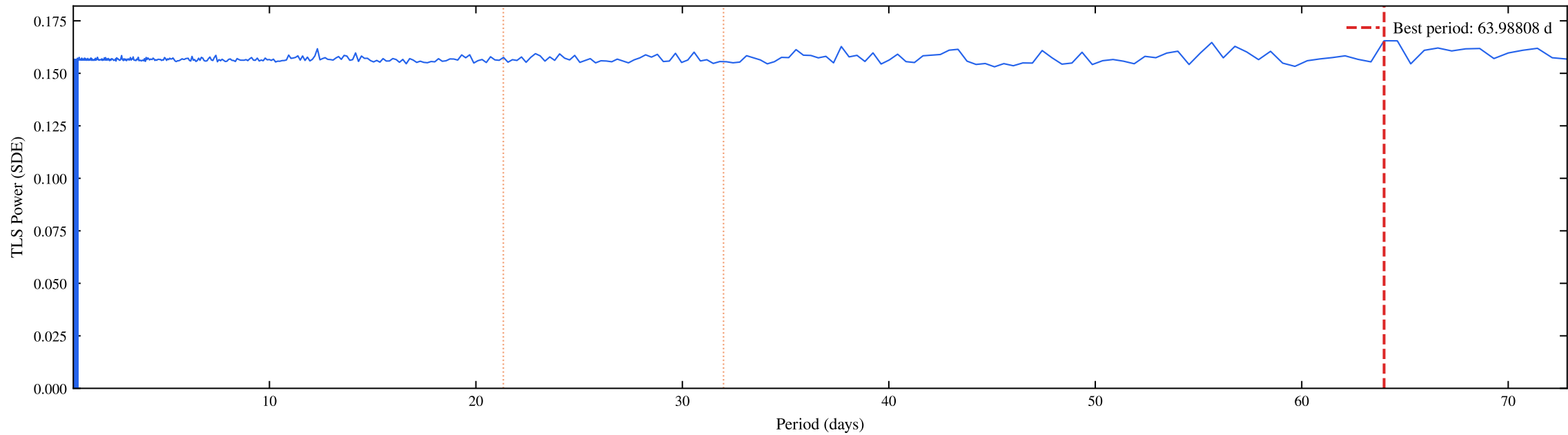
TIC 287196418 | Sectors: 53, 54, 55, 56, 57, 58, 59, 60 | TLS Periodogram (Planet 2 Search) (SDE = 0.17)
