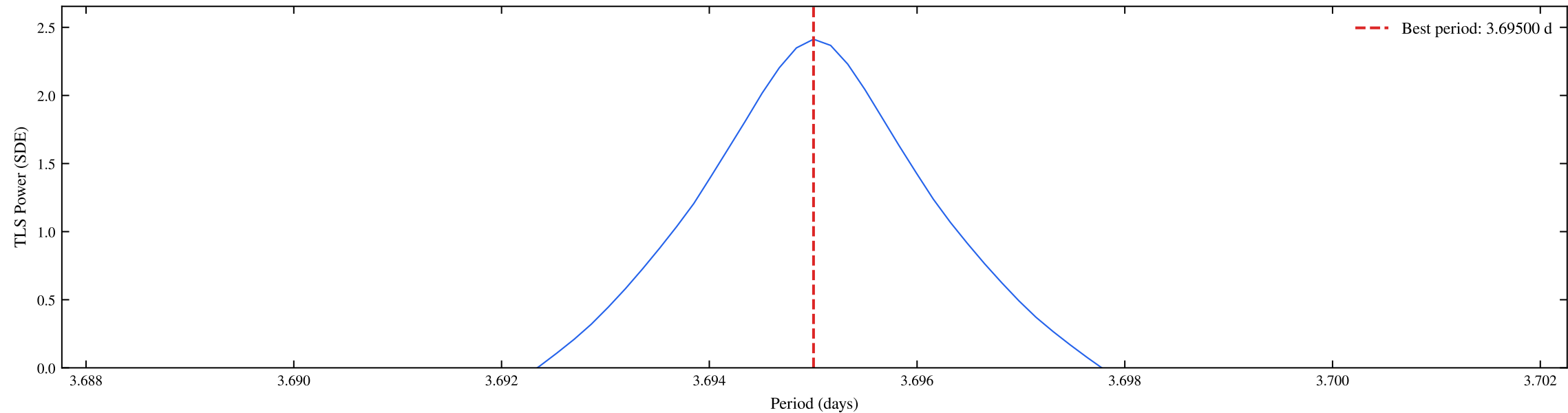
TIC 287196418 | Sectors: 53, 54, 55, 56, 57, 58, 59, 60 | TLS Coarse Periodogram (SDE = 2.41)
