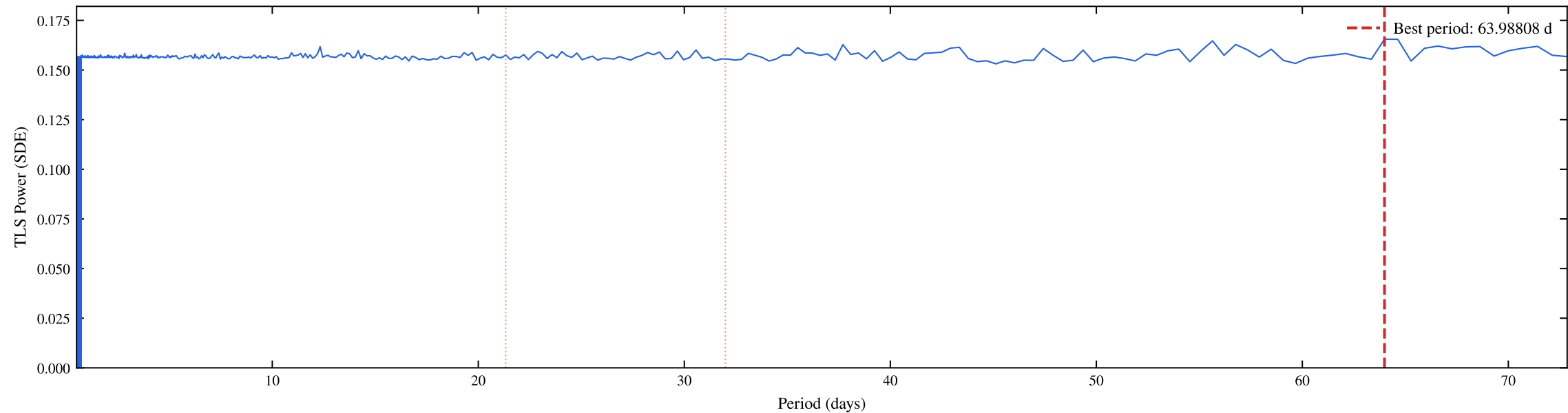
TIC 287196418 | Sectors: 53, 54, 55, 56, 57, 58, 59, 60 | TLS Coarse Periodogram (SDE = 0.17)
