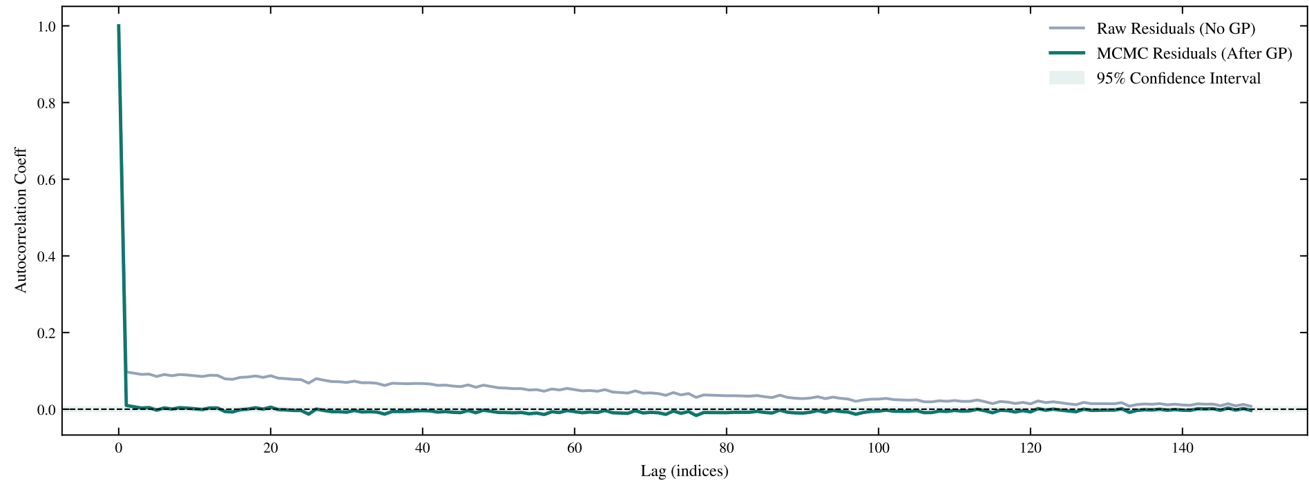
TIC 287196418 | Sectors: 53, 54, 55, 56, 57, 58, 59, 60 | GP Residuals Autocorrelation Function (ACF)
