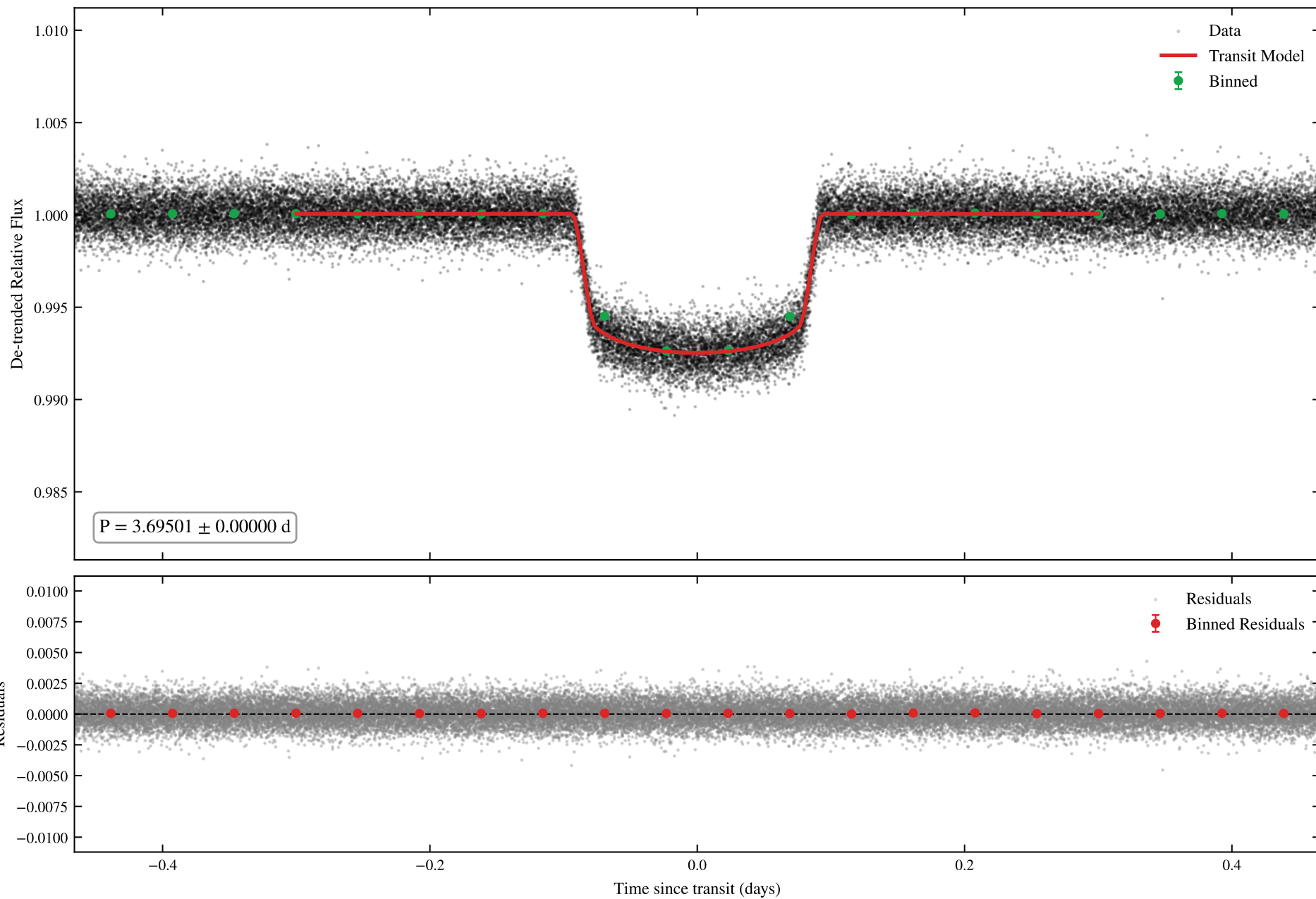
TIC 287196418 | Sectors: 53, 54, 55, 56, 57, 58, 59, 60 | Phased MCMC Fit - Planet 1
