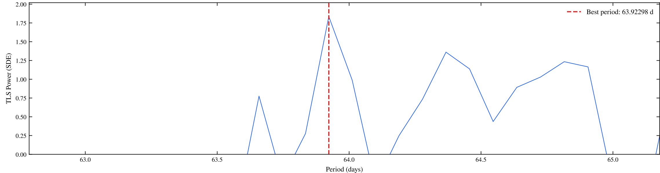
TIC 287196418 | Sectors: 53, 54, 55, 56, 57, 58, 59, 60 | TLS Fine Periodogram (SDE = 1.84)
