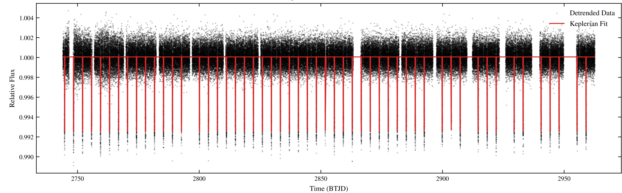
Detrended Light Curve & Best-Fit Transit Model
